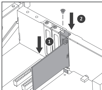
Low-profile bracket
