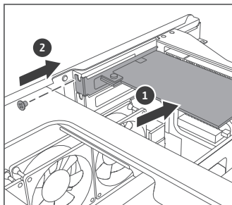
Full-height bracket
