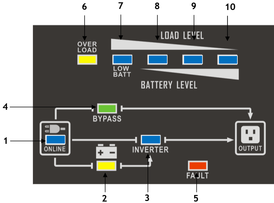
Figure 3 - Led Panel
