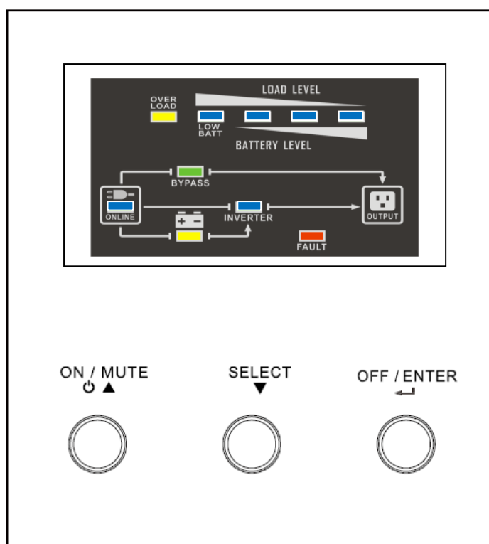
Figure 2 - Front panel
