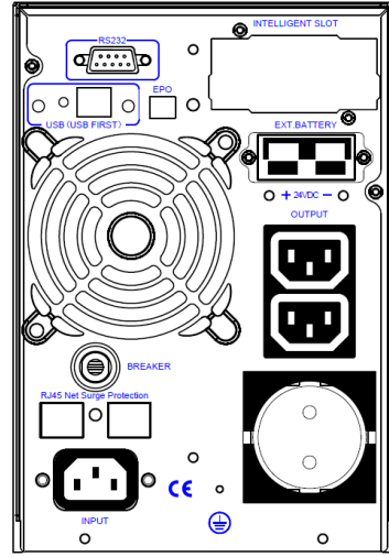
Fig. 2 Vista posteriore UPS MISSION 1000
