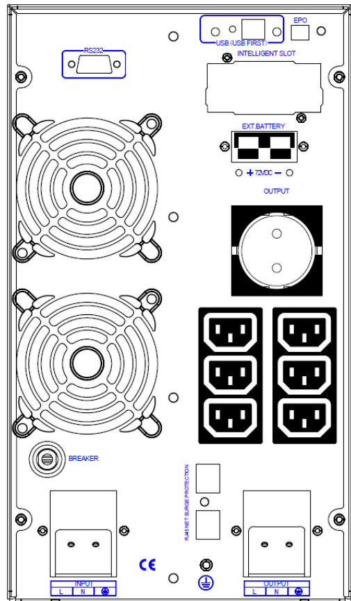
Fig. 4 Vista posteriore UPS MISSION 3000
