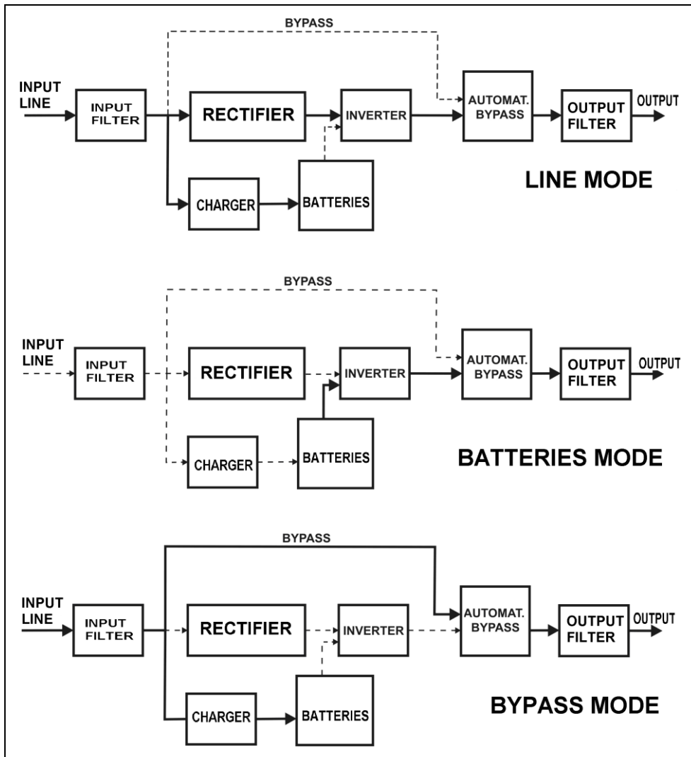
Figure 1 - Operating modes
