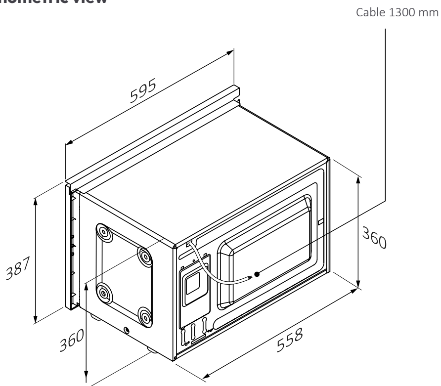
Back axonometric view
