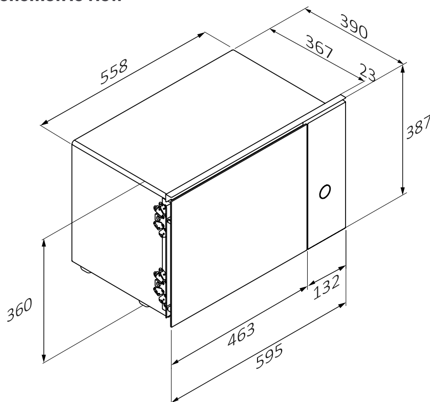
Frontal axonometric view
