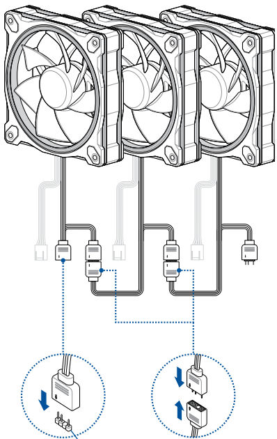
Motherboard ARGB header
